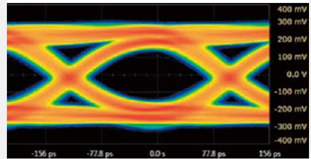
D-PHY TX Output Waveforms at 4.5 Gbps
