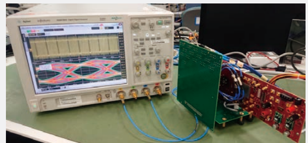
PCI Express Gen3 Evaluation Environment
