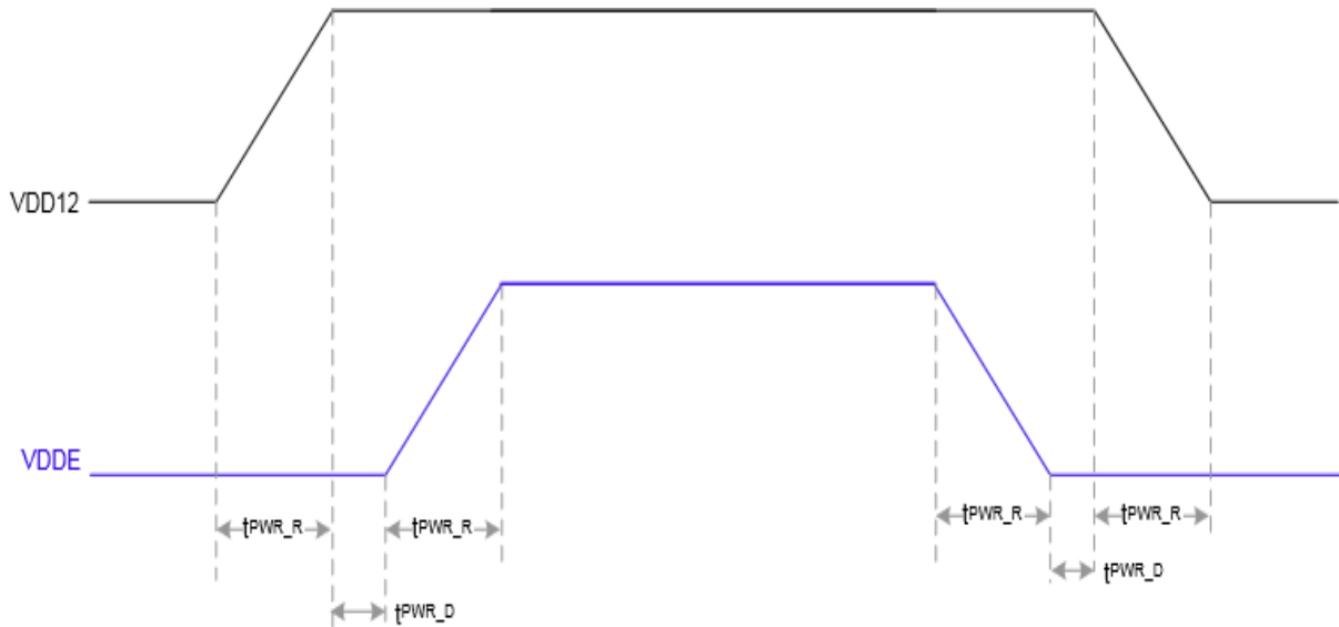
Figure 2.3. : Power-On Sequence
