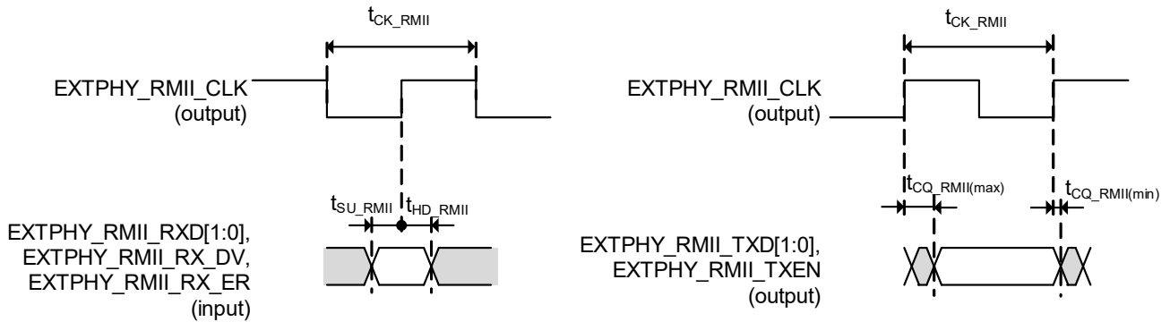
Figure 2.20. : AC Timing RMII (external PHY)
