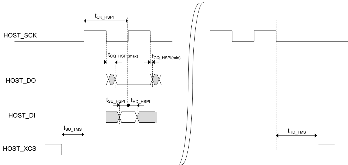
Figure 2.10. : Timing SPI interface
