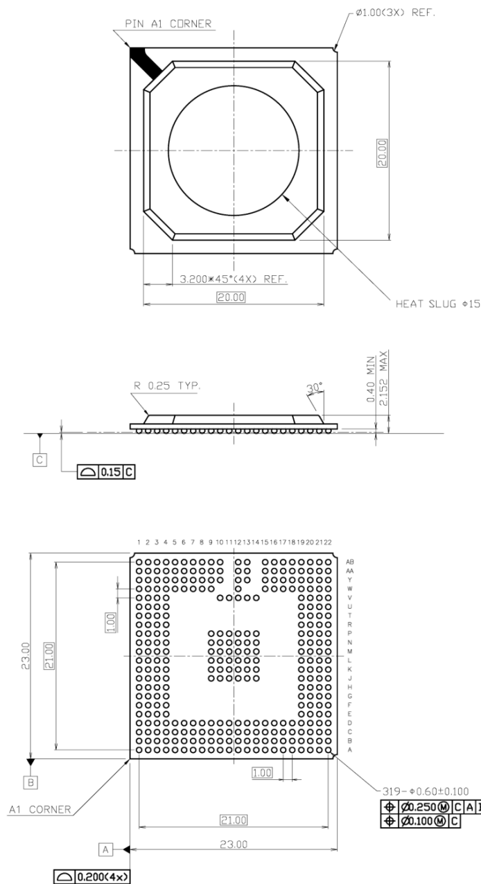
Figure 1.4. : SC1701BK3-200 Package
