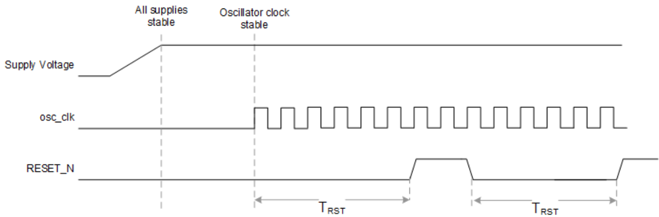
Figure 2.2. : Reset Timing
