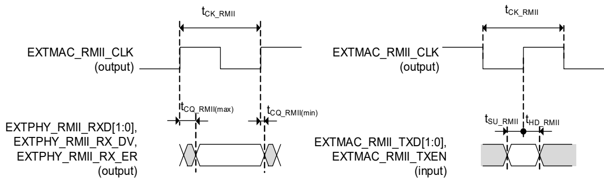
Figure 2.21. : AC Timing RMII (external MAC)
